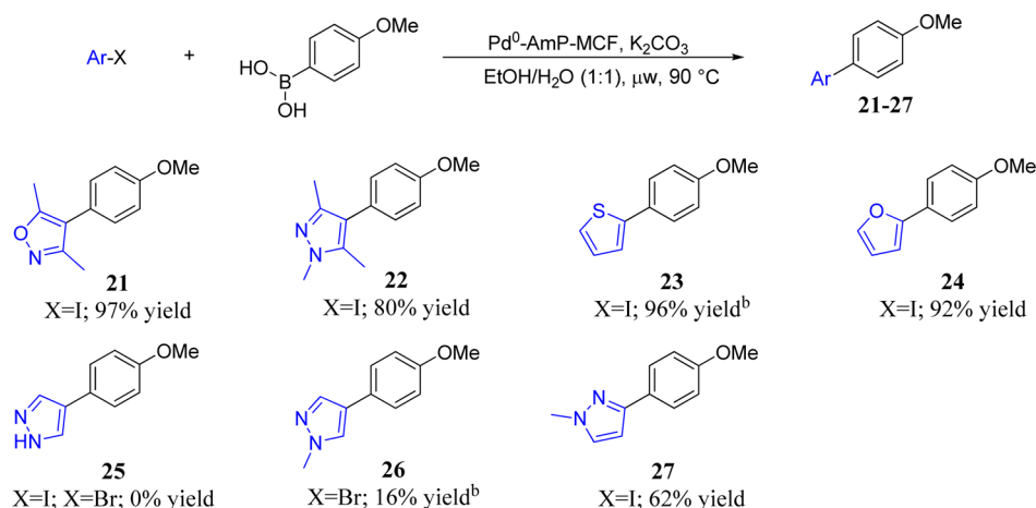
Scheme 4. Suzuki Couplings with Five-Membered Heteroaryl Halides and 4-Methoxyboronic Acid Using Pd 0 -AmP-MCF as Catalyst a
