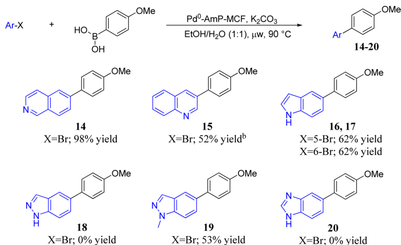
Scheme 3. Suzuki Couplings of Fused Heteroaryl Bromides and 4-Methoxyphenylboronic Acid Using Pd 0 -AmP-MCF as Catalyst a
